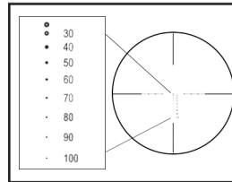
New FAST POINT 100 yard reticle
